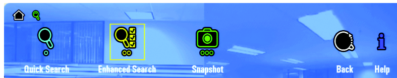
Figure 26. Search/Export Menu
